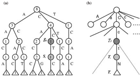
Fig. 3. (a) Suffix trie S (four-factor trie) for the sequence AACACCTCAG when l = 4 . e.g. node S_\gamma represents the substring CC and its child node S_\beta represents the substring CCT where the prefix of CCT is CC. (b) Category tree T when l = 4 .
