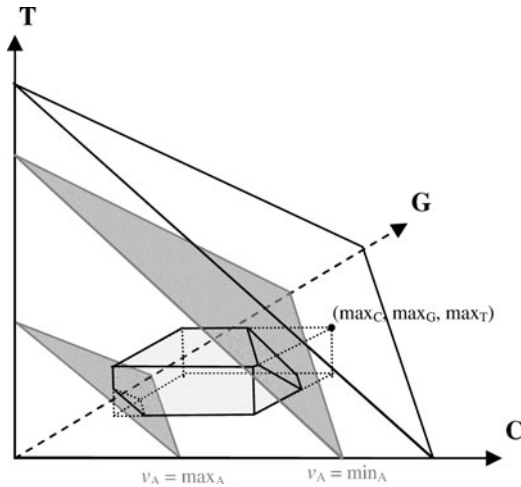
Fig. 2. Graphical representation of a partition of column vectors.
