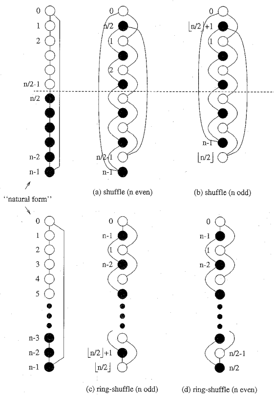
Fig. 2. Shuffle operations.
