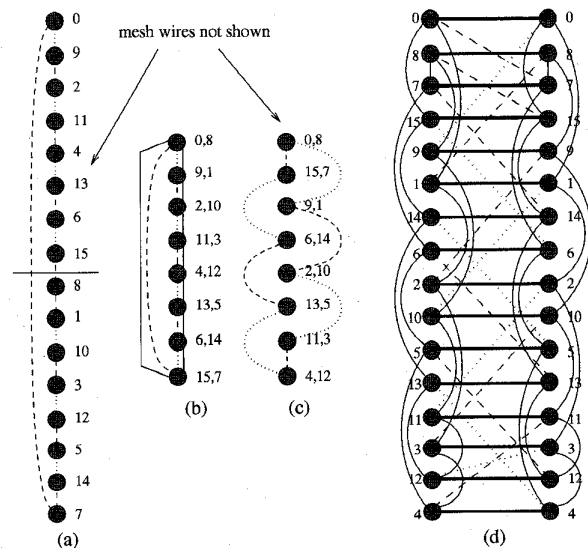
Fig. 11. Case 3— b even ( b = 8 ).
