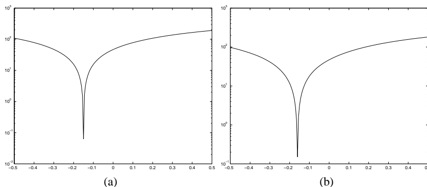
Fig. 8. Plot of the cost function (20) for a pair of images in the sequence. (a)/(b) Cost function for a pair of corresponding epipolar tangencies near the top/bottom of the profile.
