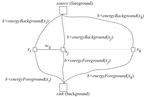
Figure 2: Graph structure for MVS problem. Each node in the graph represents a voxel. Two nodes are connected if the corresponding voxels are 6-neighbor of each other. The weight of the link between two connected nodes is defined by the dissimilarity measure \rho(x) computed at the midpoint between the centers of the corresponding voxels. All nodes are also connected to two special nodes, namely the source and the sink, with weights of the links defined as b \times energyBackground(x_i) and b \times energyForeground(x_i) respectively.
