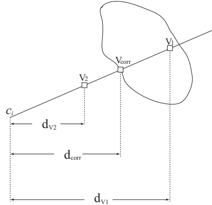
Figure 1: Consider a ray originated from the camera center c_i of view I_i that passes through the bounding box. Along this ray, the score C(V_{corr}) for voxel V_{corr} is a maximum, and hence the depth corresponding to V_{corr} is the estimated correct depth, denoted by d_{corr} . Voxel V1 has a depth d_{V1} which is larger than d_{corr} . V1 is therefore deemed to be invisible in view I_i as it is occluded by the voxel V_{corr} . On the contrary, voxel V2 has a depth d_{V2} which is smaller than d_{corr} . V2 is therefore deemed to be visible in view I_i . In this case, B\_VOTE_i(V2) = 1 and B\_VOTE_i(V1) = 0 .
