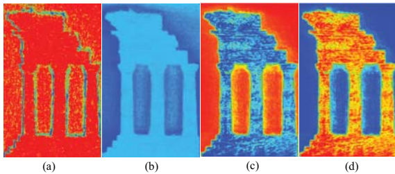
Figure 3: Comparison between the proposed foreground / background energy and the intelligent ballooning term proposed in (Hernández et al., 2007). From left to right: (a) photo-consistency energy, (b) intelligent ballooning term, (c) proposed foreground energy, and (d) proposed background energy. Blue color indicates a low energy value and red color indicates a high energy value. Note that the foreground energy values are lower inside the object and higher outside the object. The background energy values, on the other hand, are higher inside the object and lower outside the object.
